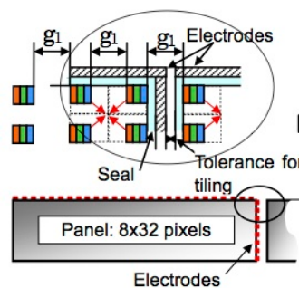
Fig.3 Usual design
